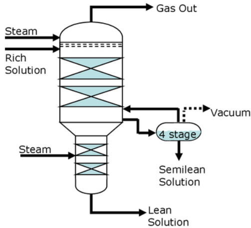
Gambar 2. Unit stripping CO 2 skala industri
